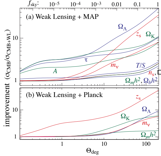
Fig. 34. The improvement of the accuracy of cosmological parameters when supplementing CMB data from WMAP (upper panel) and the Planck satellite (lower panel) by a cosmic shear survey of solid angle \theta^2\pi . The accuracies are significantly improved, certainly when combined with WMAP, but even in combination with Planck, the accuracies of the density parameters can be increased, when using next-generation cosmic shear surveys with hundreds of square degrees (from Hu & Tegmark 1999)
